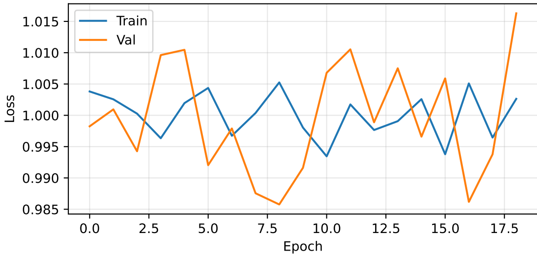
Losses: ddpm_evaluation_20250813_000400
